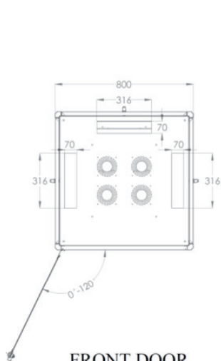
FRONT DOOR OPENING ANGLE
