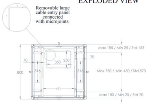
EXPLODED VIEW
